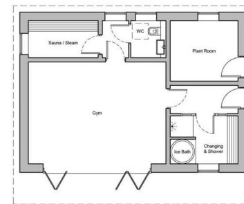
Ground Floor Plan GFA - 68.8m 2 (7,397sqft)
